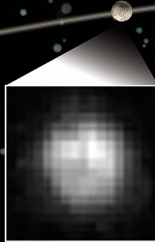
Hubble Space Telescope Image
